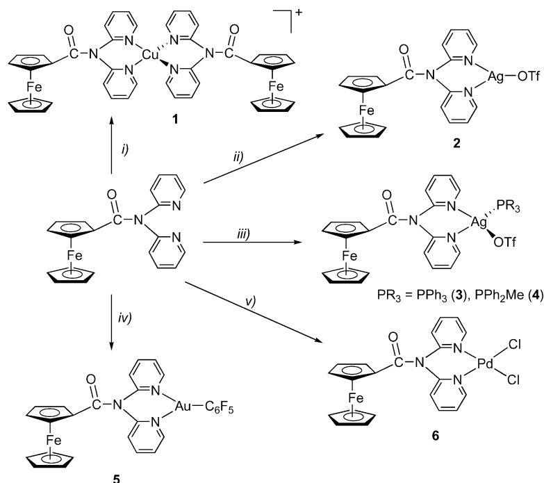
Scheme 1. (i) 1/2 [Cu(NCMe) 4 ]PF 6 , (ii) Ag(OTf), (iii) [Ag(OTf)(PR 3 )], (iv) [Au(C 6 F 5 )(tbt)], (v) [PdCl 2 (NCPh) 2 ].
