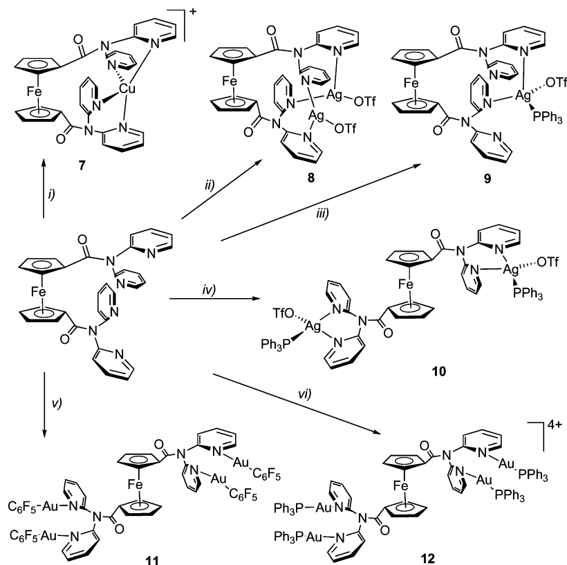
Scheme 2. (i) 1/2 [\text{Cu}(\text{NCMe})_4]\text{PF}_6 , (ii) 2 \text{ Ag}(\text{OTf}) , (iii) [\text{Ag}(\text{OTf})(\text{PPh}_3)] , (iv) 2 [\text{Ag}(\text{OTf})(\text{PPh}_3)] , (v) 4 [\text{Au}(\text{C}_6\text{F}_5)(\text{ttht})] , (vi) 4 [\text{Au}(\text{OTf})(\text{PPh}_3)] .
