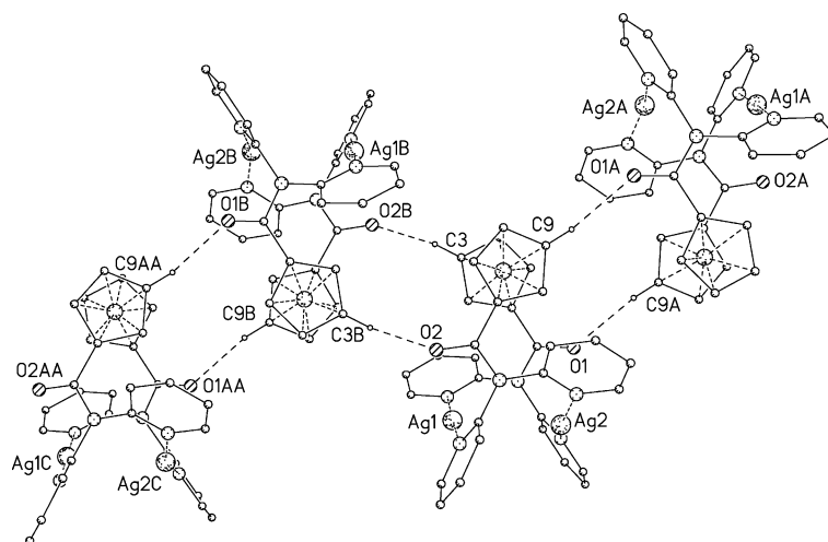
Figure 6. Formation of chains through hydrogen bonding (dotted lines) in complex 8 .
