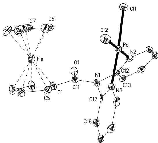
Figure 3. Molecular structure of complex 6 showing the atom-numbering scheme. Displacement parameter ellipsoids represent 50% probability surfaces. Hydrogen atoms and solvent molecules have been omitted for clarity.
