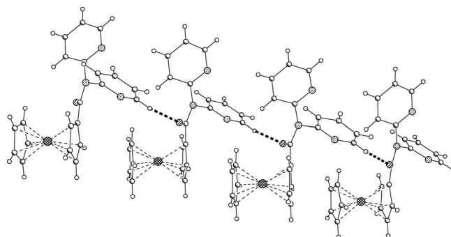
Figure 1. Formation of chains through hydrogen bonds (dotted lines) in L1 .
