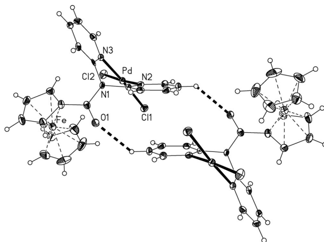
Figure 4. Some hydrogen bonds in complex 6 .
