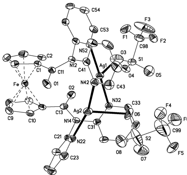
Figure 5. Molecular structure of compound 8 showing the atom-numbering scheme. Displacement parameter ellipsoids represent 30% probability surfaces. Hydrogen atoms have been omitted for clarity. Only one position of the disordered triflate group is shown.
